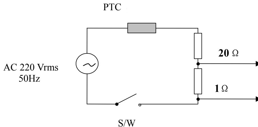
Fig. 1 Test circuit
